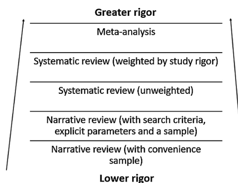
Fig. 2. A scale of rigorous methods for literature reviews.
